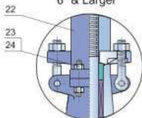
Yoke for 6" & Larger
