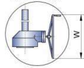
Gear Standard for 26" & Larger
