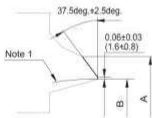
Wall Thickness not Over 0.88in (22mm) Welding End Detail for Joint Without Backing Ring
