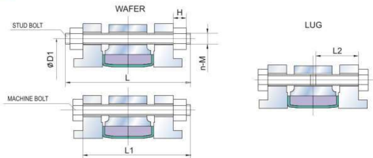
RECOMMENDED BOLT LENGTHS FOR CONCENTRIC BUTTERFLY VALVE
