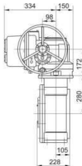
Overall Dimensions &amp; Weight of Electric Actuator
