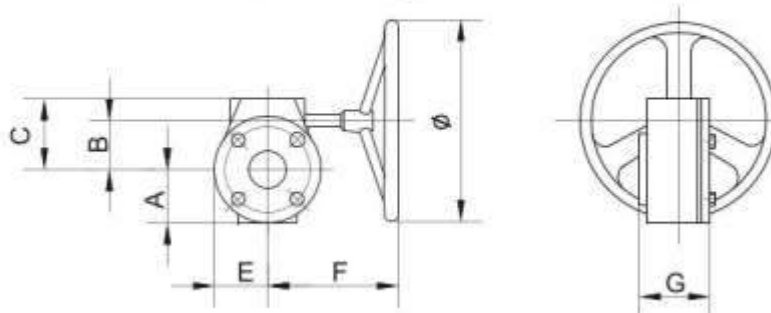
Overall Dimensions &amp; Weight of Worm Gear Actuator
