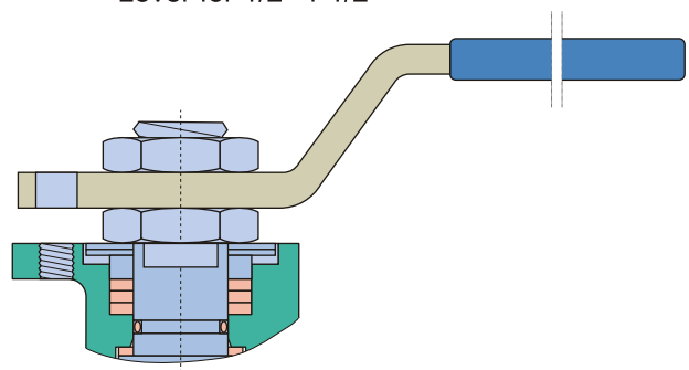
Lever for 1/2"-1 1/2"
