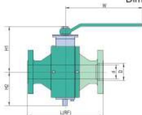
Full Bore
