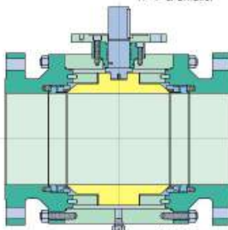
TF 6" & Larger
