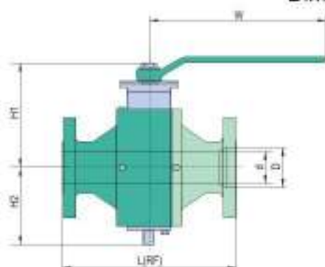
Full Bore
