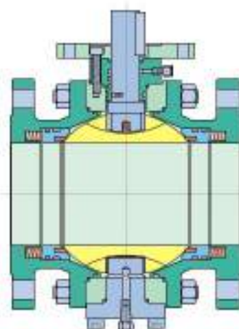
TF 4" & Smaller
