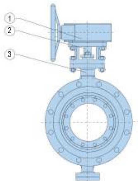
Triple Eccentric Design Construction. UNI DIRECTIONAL
