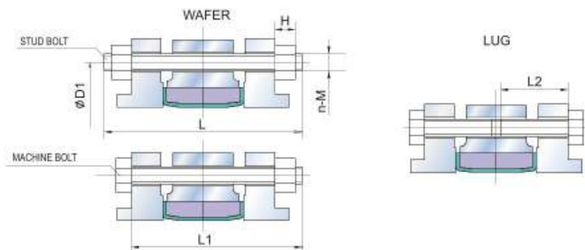
RECOMMENDED BOLT LENGTHS FOR CONCENTRIC BUTTERFLY VALVE
