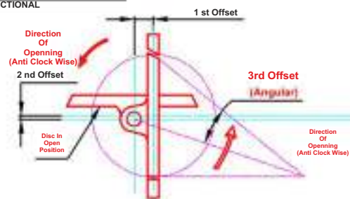
Triple Eccentric Design Construction. UNI DIRECTIONAL
