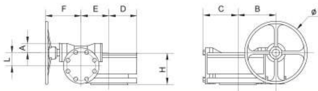
Overall Dimensions &amp; Weight of Double-Stage Worm Gear Actuator
