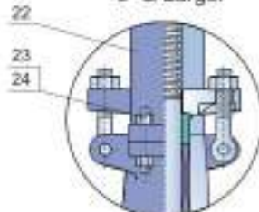
Yoke for 8" &amp; Larger
