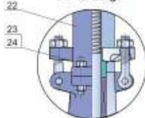
Yoke for 14" &amp; Larger
