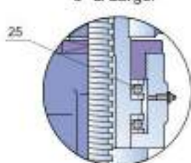
Bearing for 6" &amp; Larger
